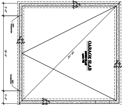
7 GARAGE FOUNDATION PLAN 1/4" = 1'-0"
