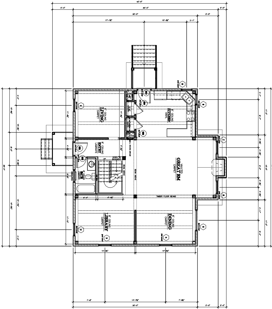
1 MAIN LEVEL FLOOR PLAN 1/8" = 1'-0"
